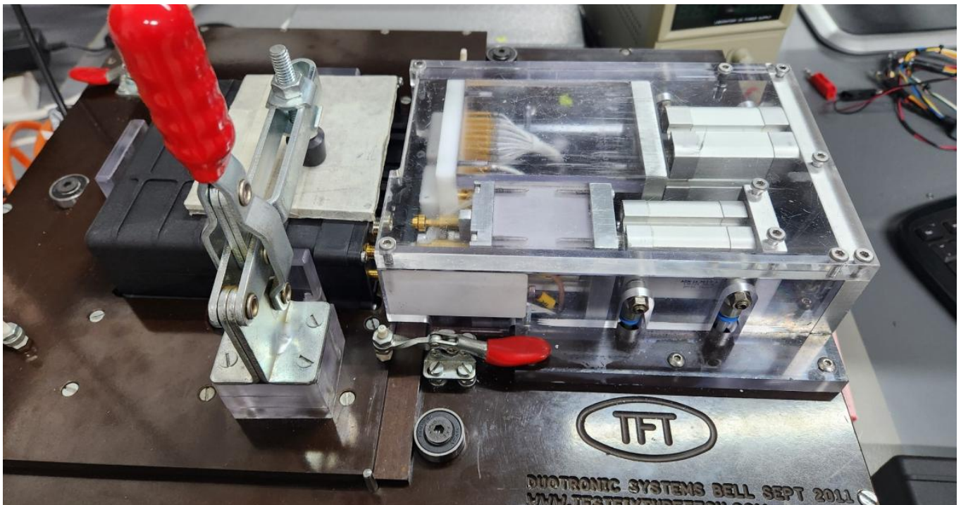
Duotronic: industrial test fixture and hardware integration.
